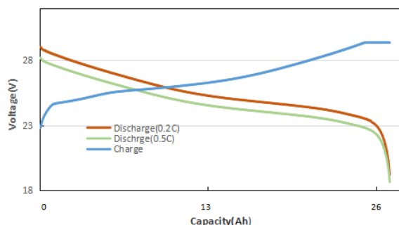
25. 2V26Ah-Charge-Discharge curve (25°C)
